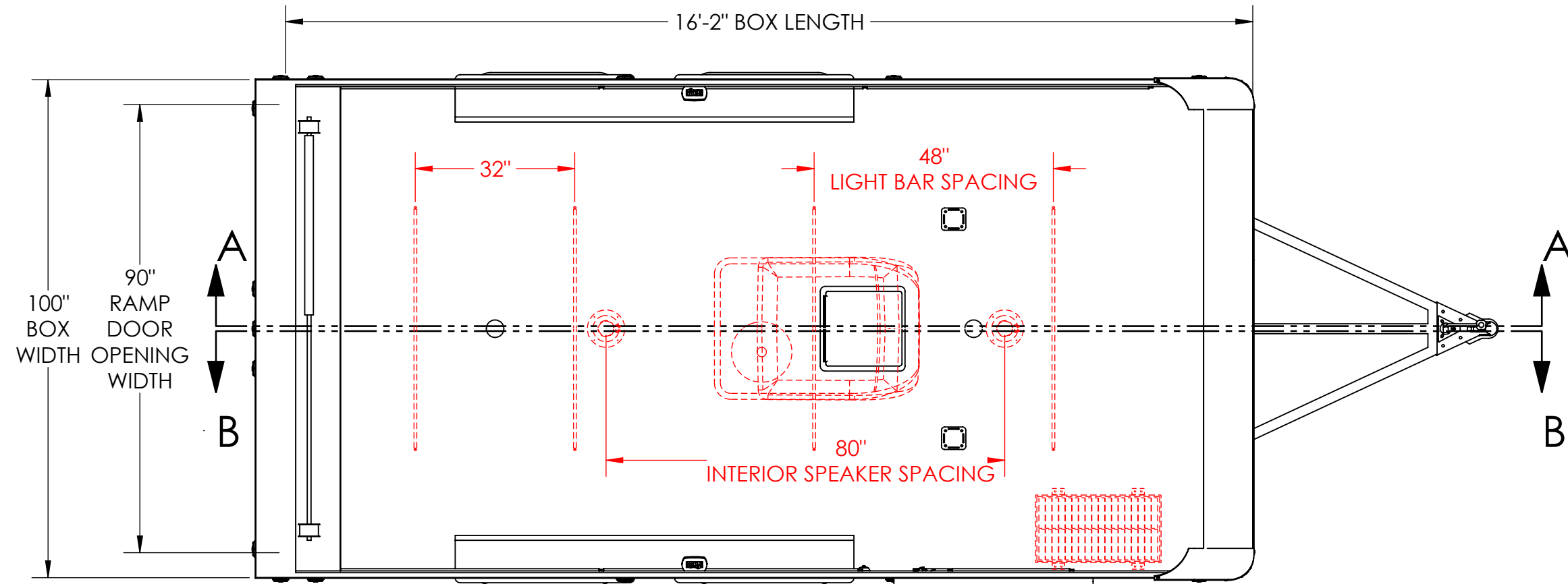
TOP VIEW ROOF & CEILING LAYOUT
