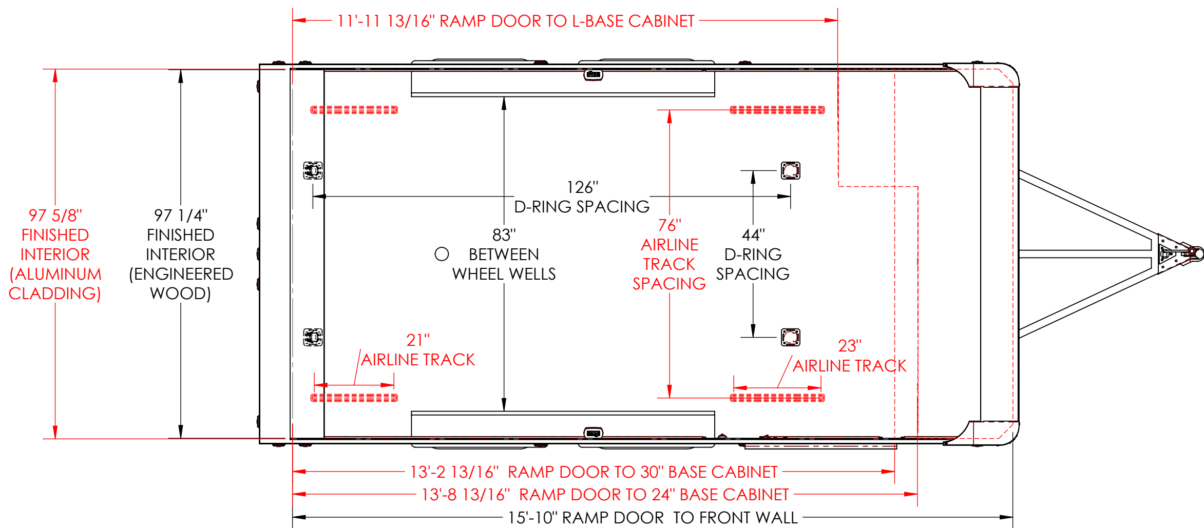
TOP VIEW FLOORPLAN LAYOUT
