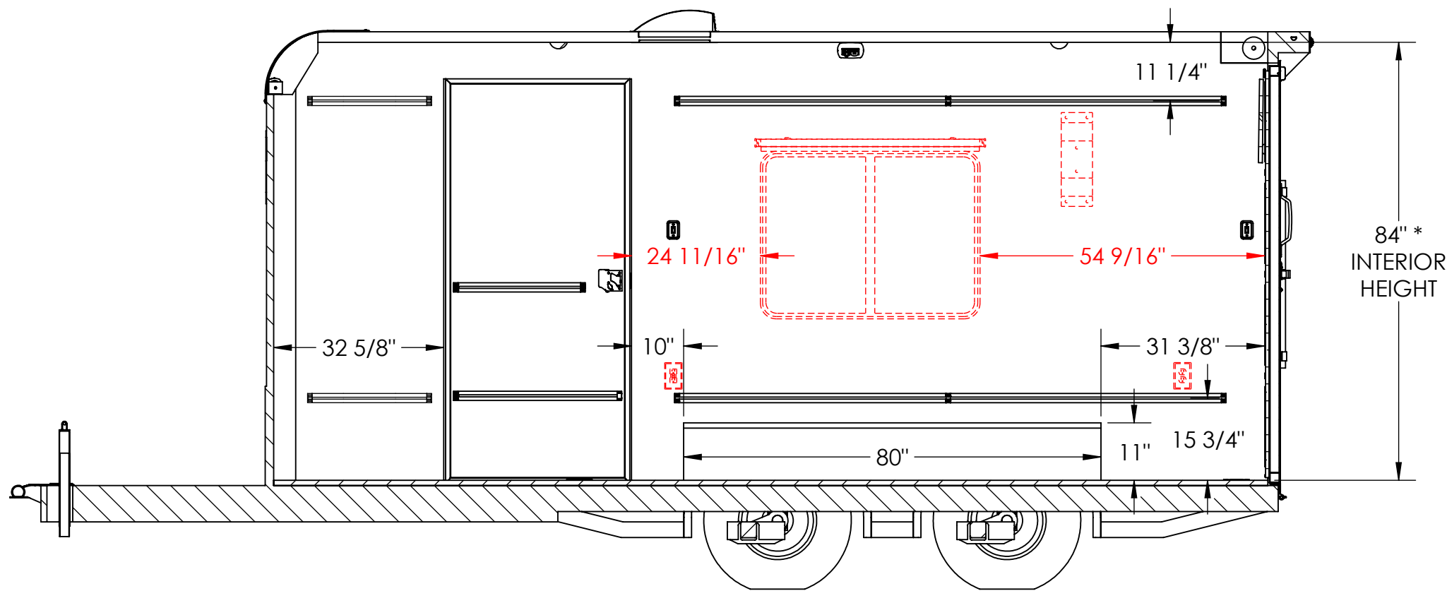
INTERIOR CURB SIDE SECTION B-B
