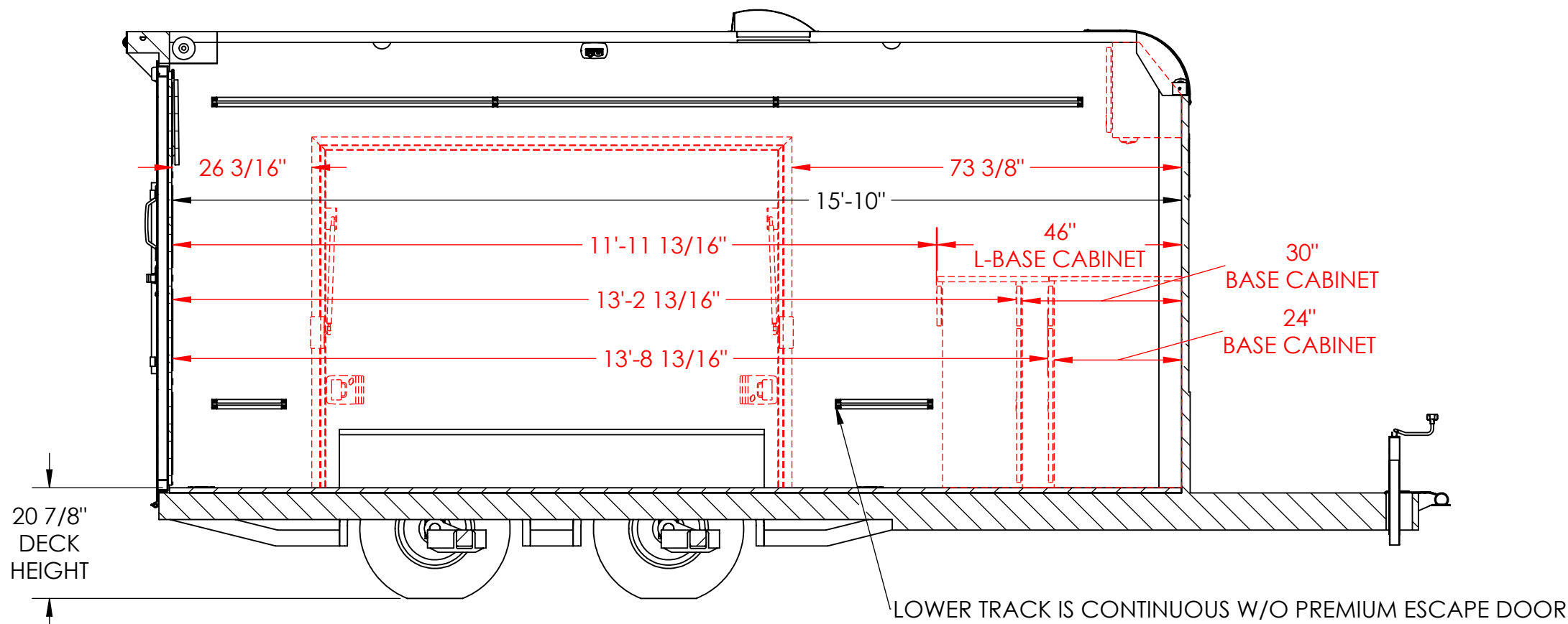
INTERIOR ROAD SIDE SECTION A-A
